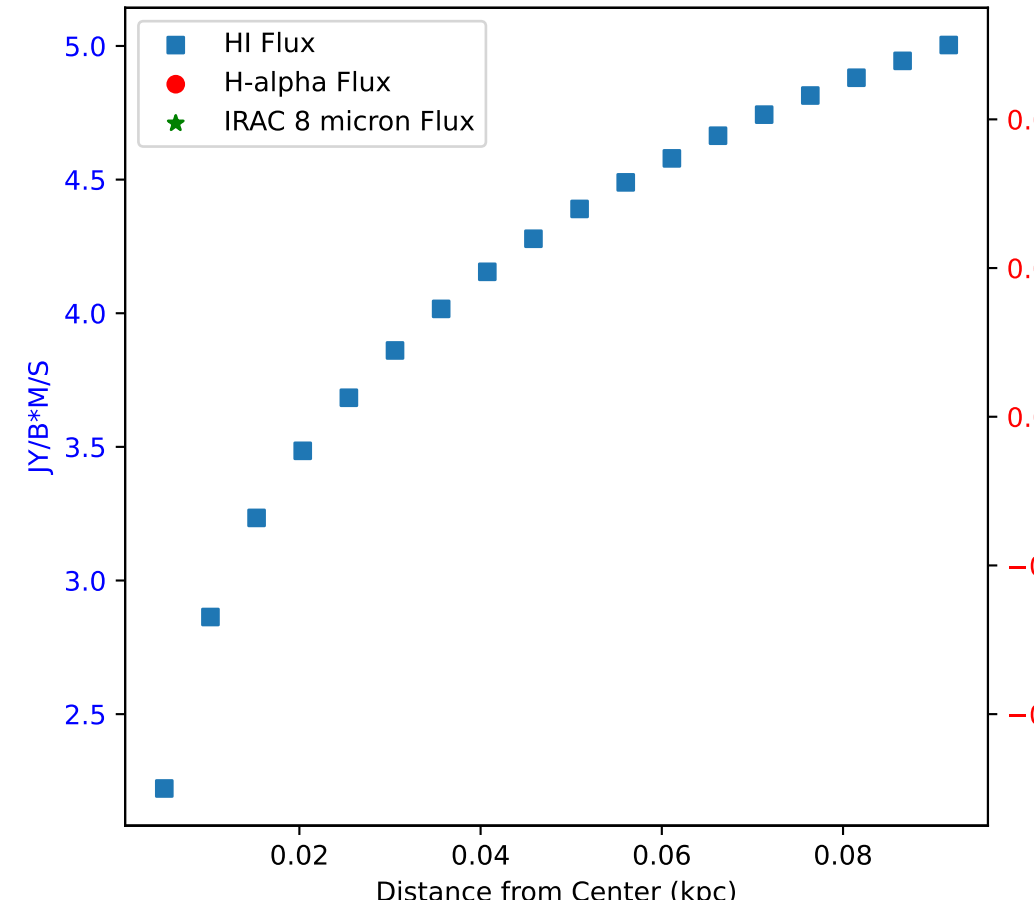
Flux of HI vs. H-alpha in Galaxy: IC10 - Region 19
