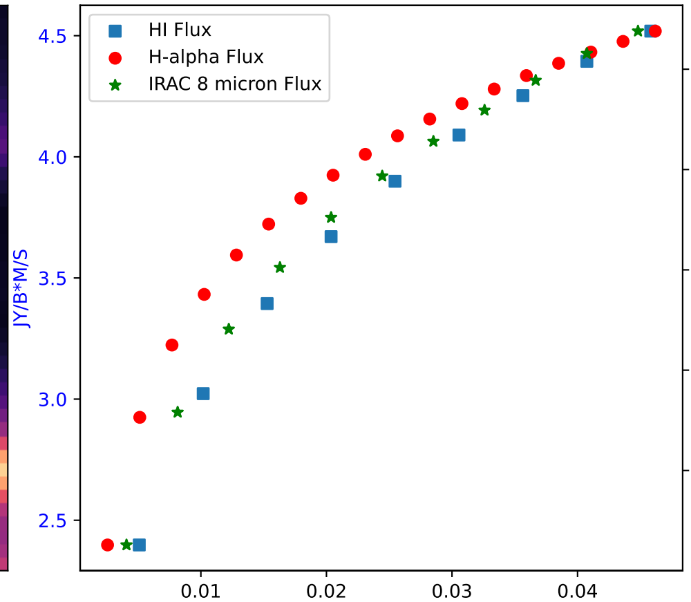
Flux of HI vs. H-alpha in Galaxy: IC10 - Region 11
