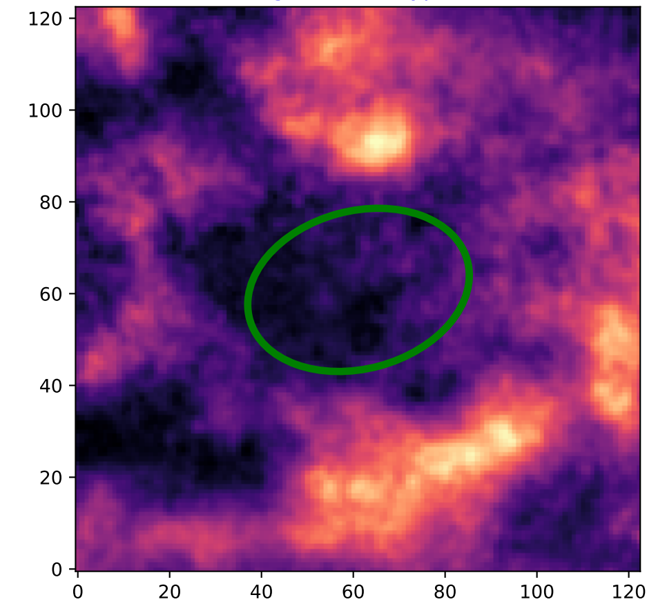
Region: 3 HI - Type 1
