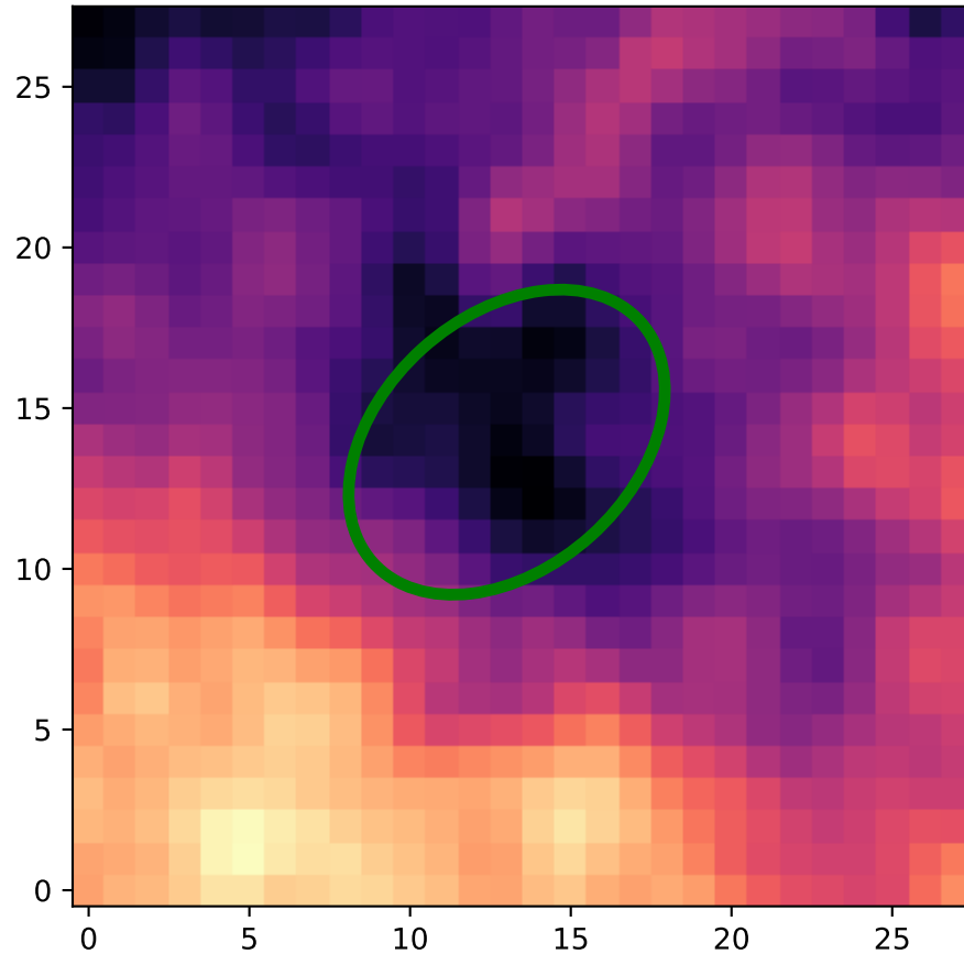
Region: 18 HI - Type 2
