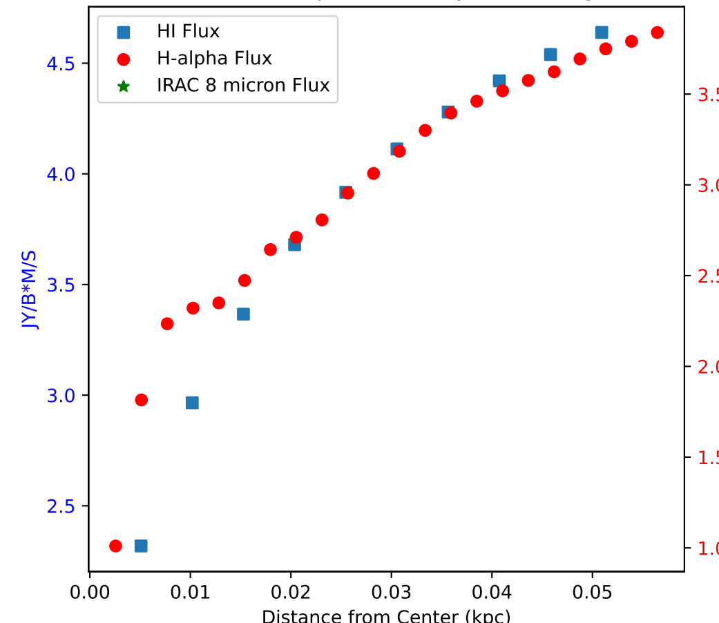
Flux of HI vs. H-alpha in Galaxy: IC10 - Region 1
