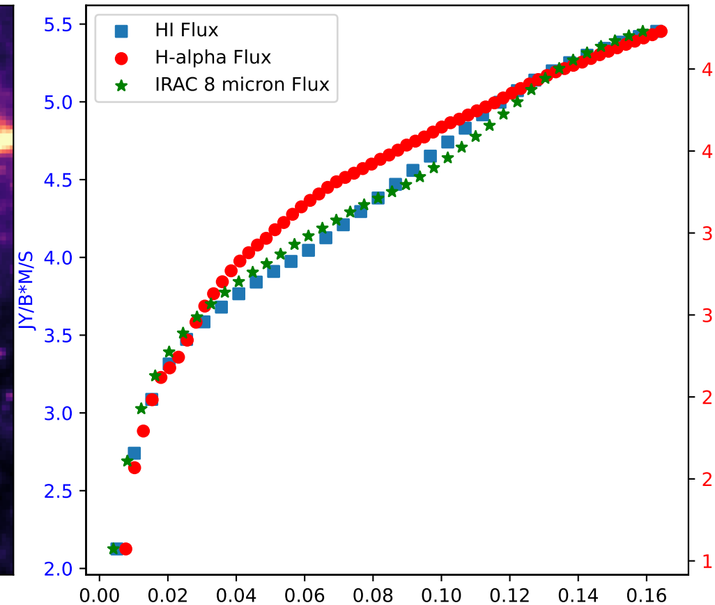
Flux of HI vs. H-alpha in Galaxy: IC10 - Region 8
