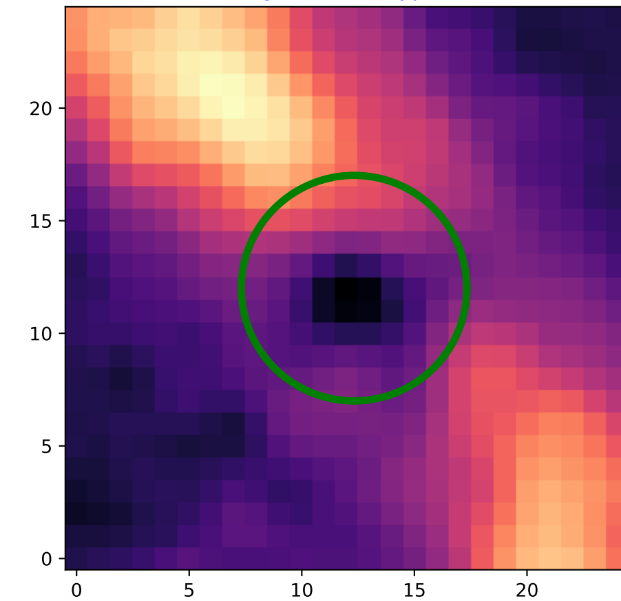
Region: 9 HI - Type 2
