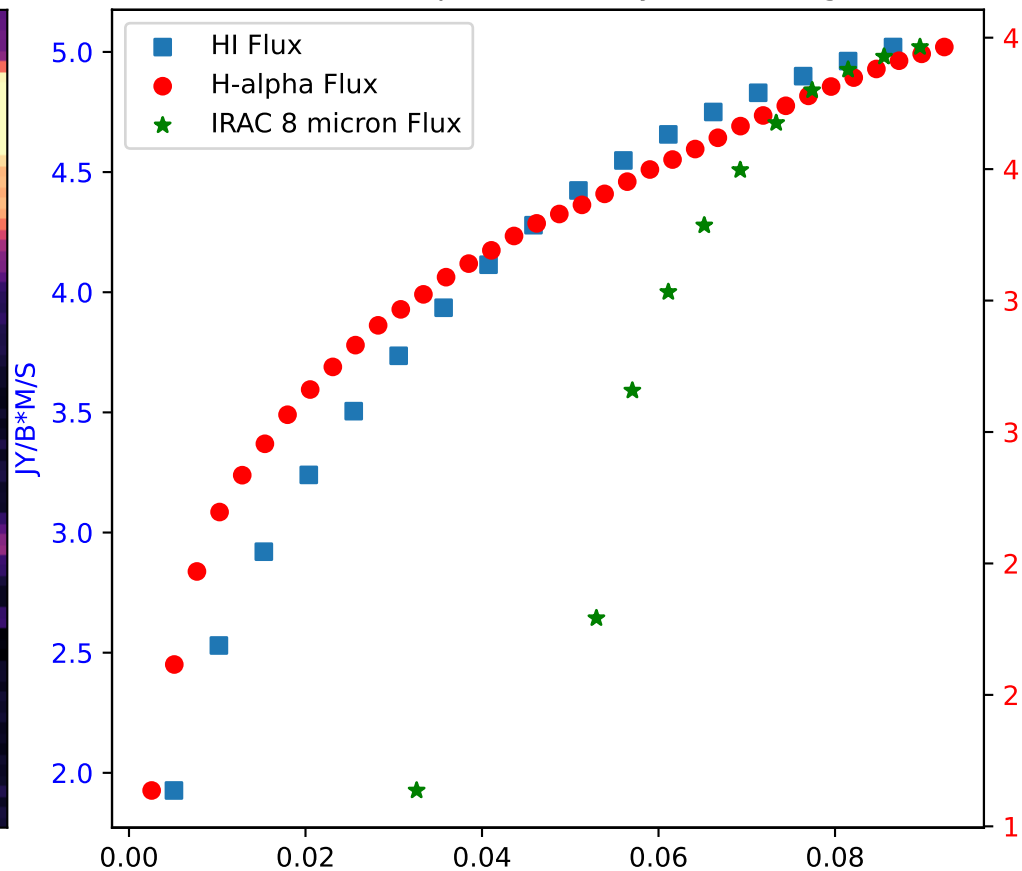
Flux of HI vs. H-alpha in Galaxy: IC10 - Region 15
