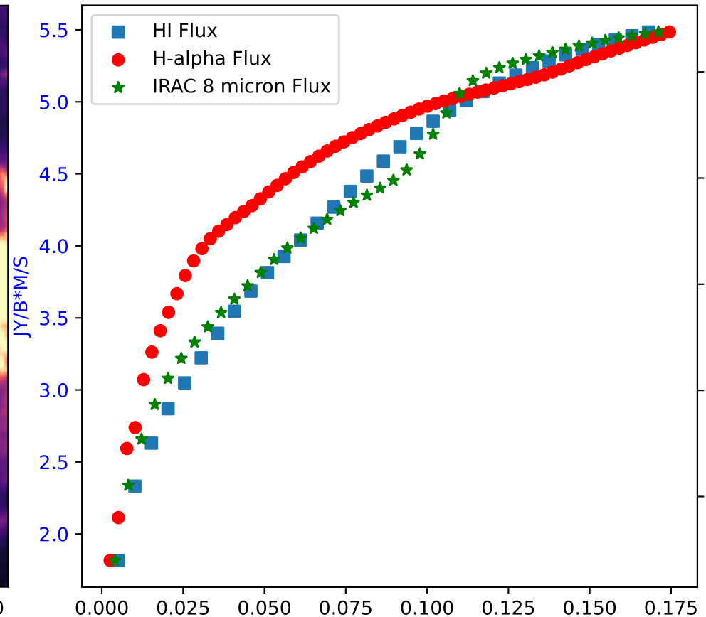
Flux of HI vs. H-alpha in Galaxy: IC10 - Region 10
