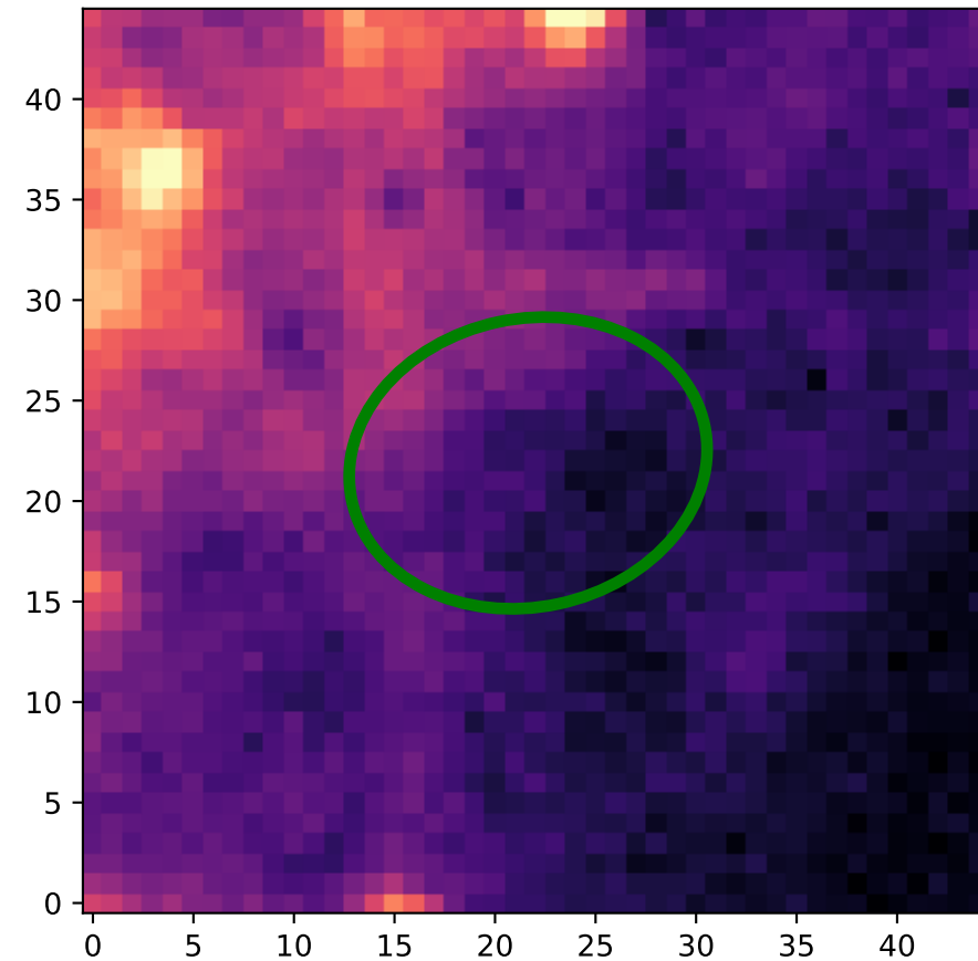
H-alpha - Classification: Bubble-Like
