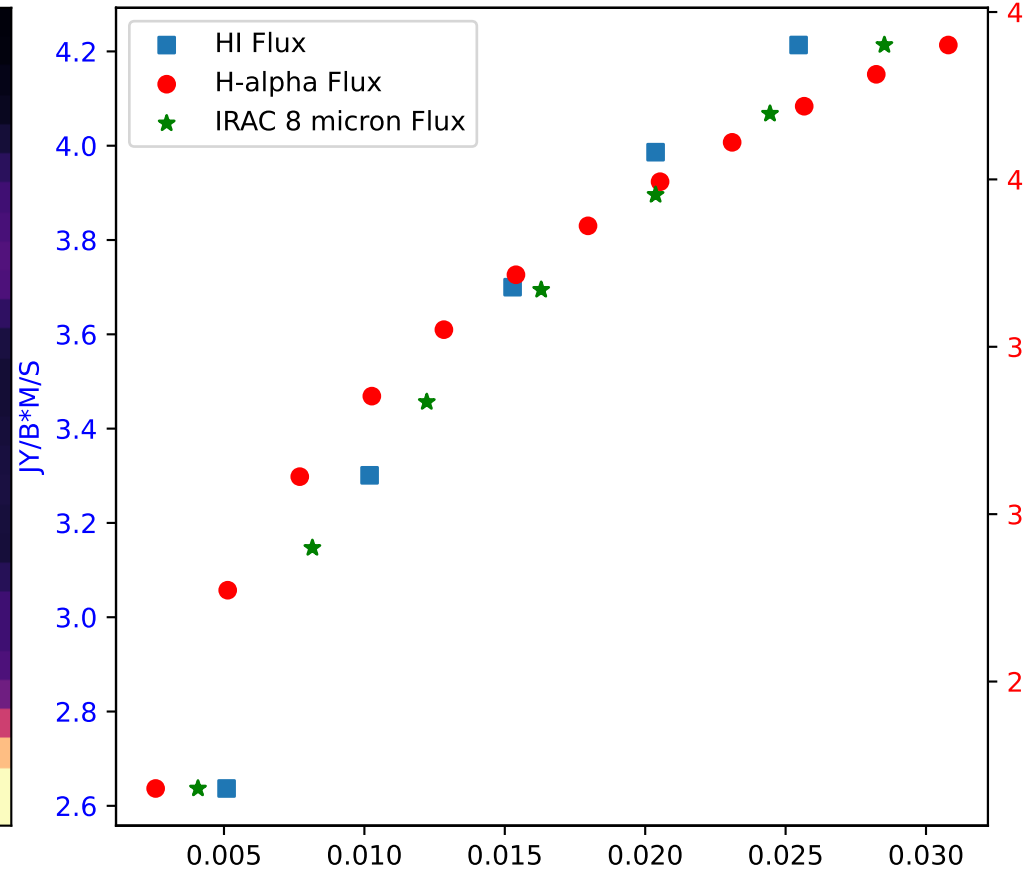
Flux of HI vs. H-alpha in Galaxy: IC10 - Region 12
