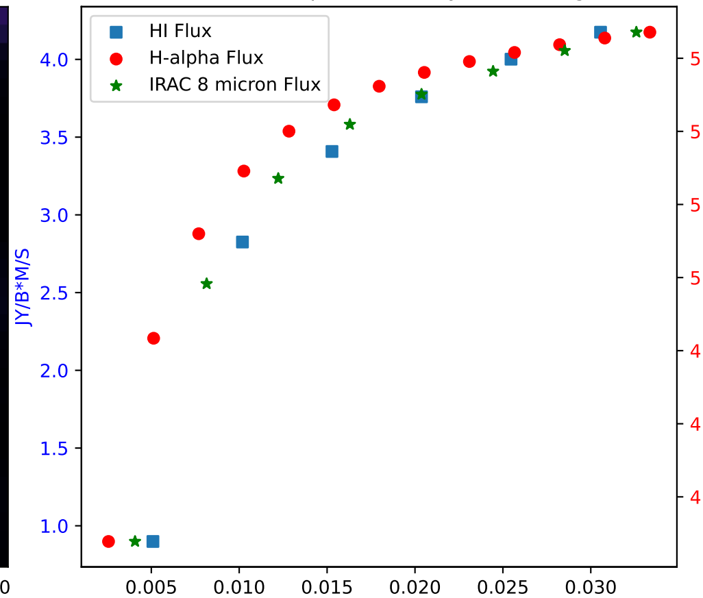
Flux of HI vs. H-alpha in Galaxy: IC10 - Region 9
