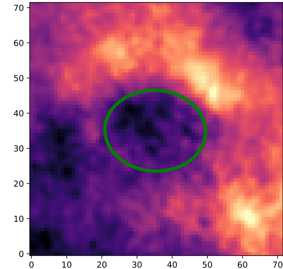
Region: 14 HI - Type 1
