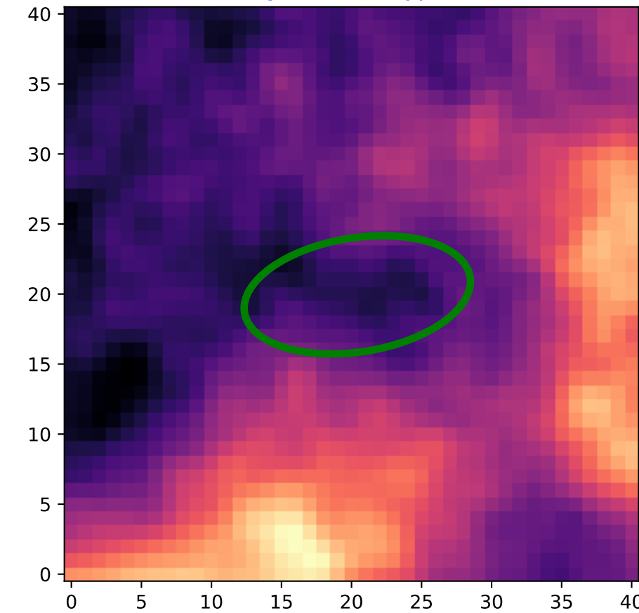
Region: 2 HI - Type 2
