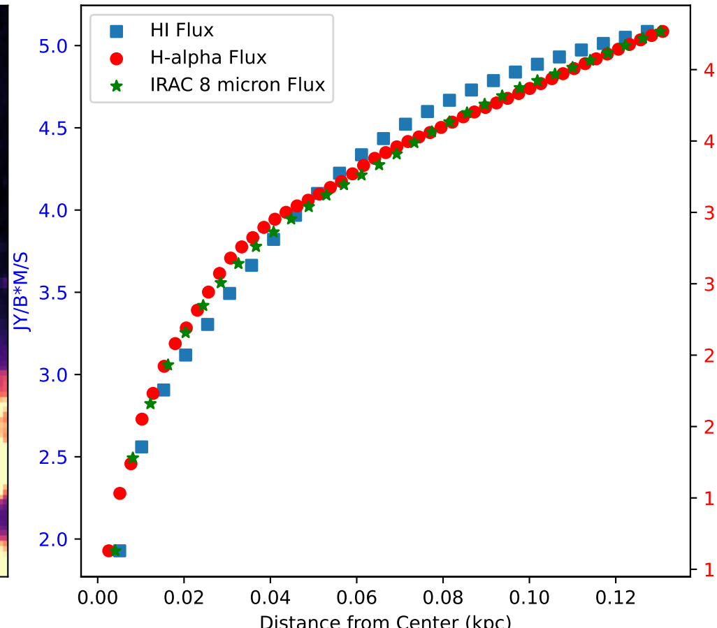
Flux of HI vs. H-alpha in Galaxy: IC10 - Region 6
