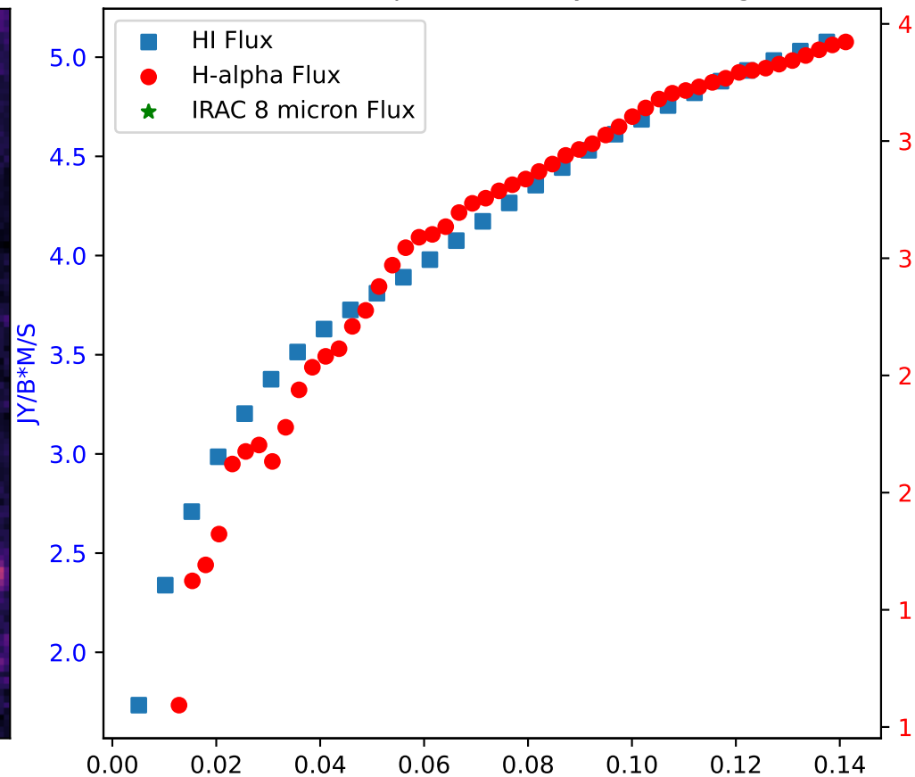
Flux of HI vs. H-alpha in Galaxy: IC10 - Region 17
