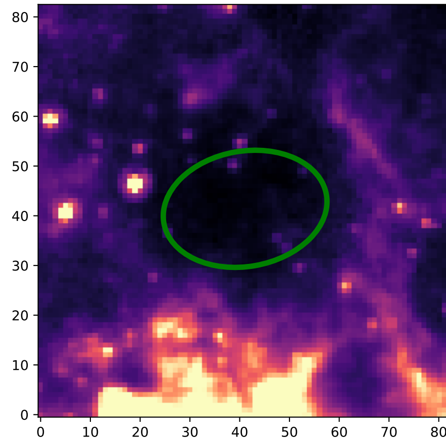
IRAC 8 micron - Classification: Bubble-Like
