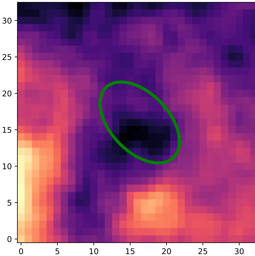
Region: 11 HI - Type 1
