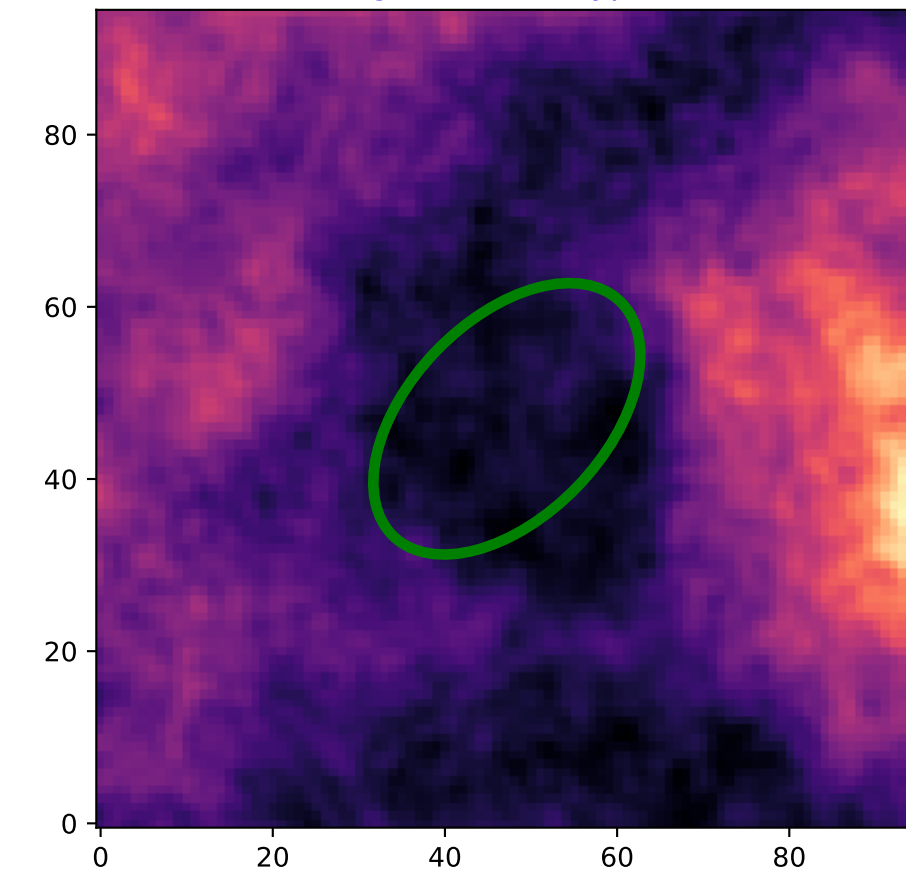
Region: 17 HI - Type 1
