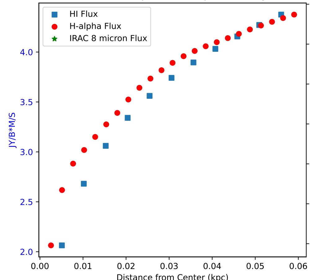
Flux of HI vs. H-alpha in Galaxy: IC10 - Region 2
