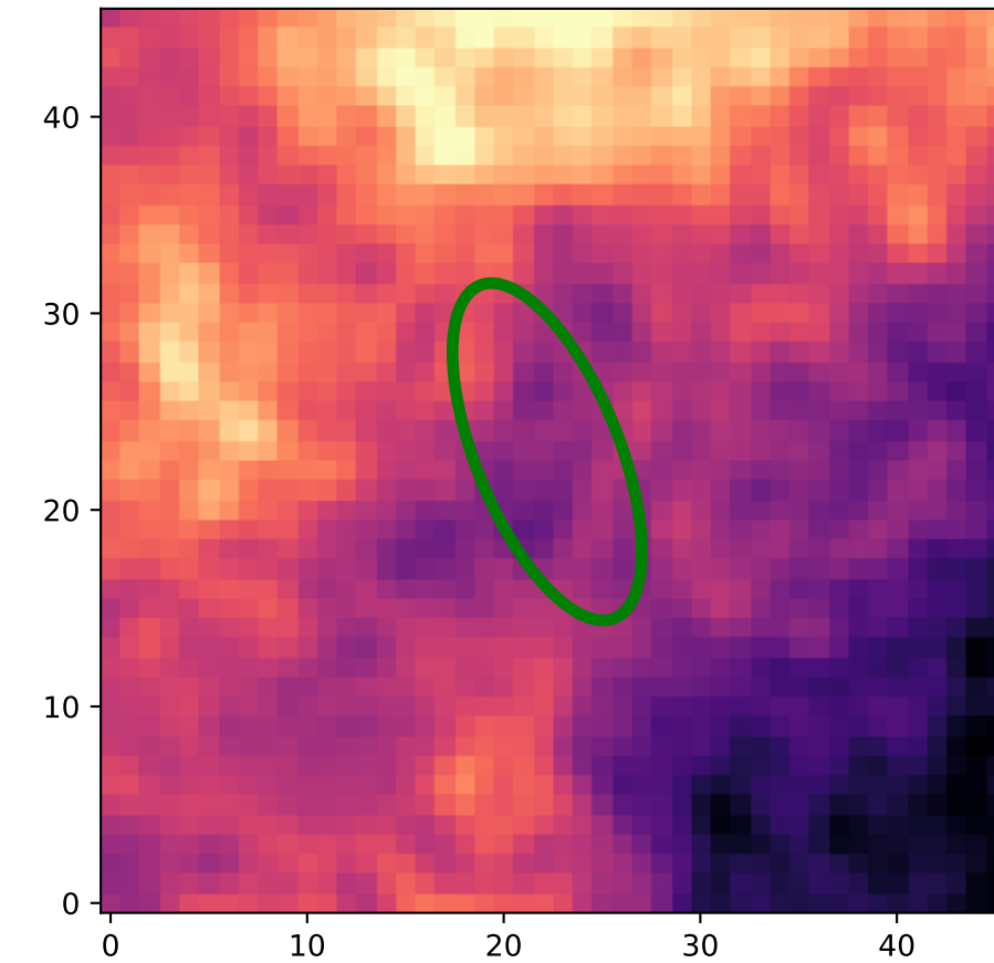
Region: 20 HI - Type 2
